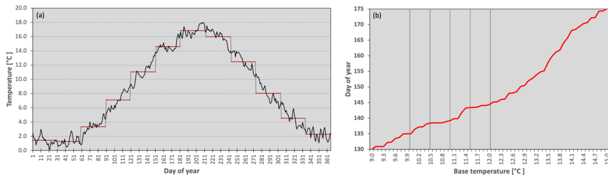
Figure 2.10. Average daily temperature and monthly temperature (left) and change of the base temperature with date (vertical lines mark 10°C, 10.5°C, 11°C, 11.5°C and 12°C, respectively), derived from the data from Ullensvang station, for the period 2001-2020.
