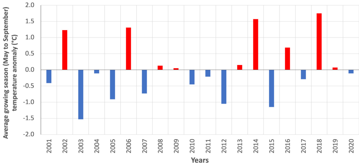
Figure 3.4. Anomalies of average temperature for May-September for each year with respect to the average temperature for May-September for the period 2001-2020, for Ullensvang.
